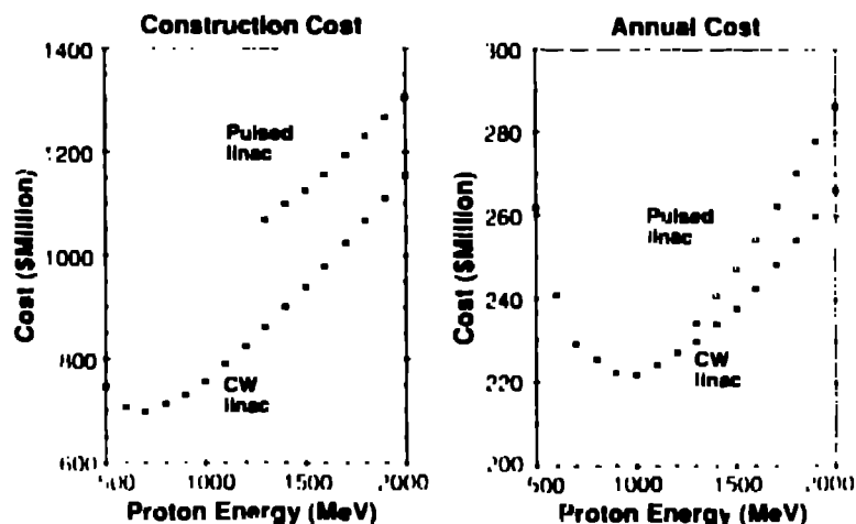
Fig. 2. ATW construction cost and annual cost versus proton energy, for cw and pulsed linac models. that parameterize the CCL costs. While the models are incomplete in terms of structural detail, the principal cost factors are included, along with the usual multipliers for contingency, project management, ED&I, etc. Results are displayed in Fig. 2, which shows the estimated construction cost and annual cost versus beam energy for cw and pulsed linacs.
